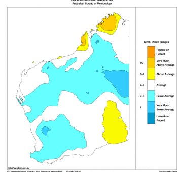
Minimum Temperature Deciles 1 October to 31 December 2022 Australian Bureau of Meteorology
